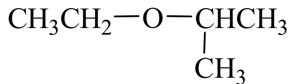
乙异丙醚
